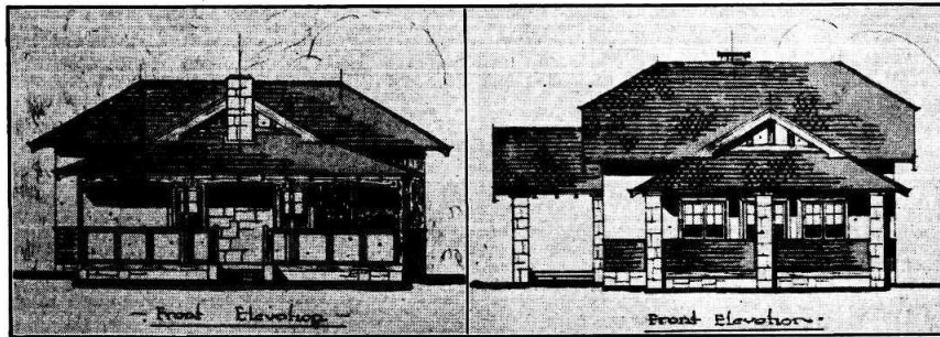
Winning entries in the Perth City Council's competition for designs for bungalows suitable for erection on the No. 3 Subdivision, at the end of the plank road, City Beach Estate. The design on the left, it is estimated, would cost under £250, and that on the right, under £300. The designer in each case was Mr. J. H. G. Hargrave.
